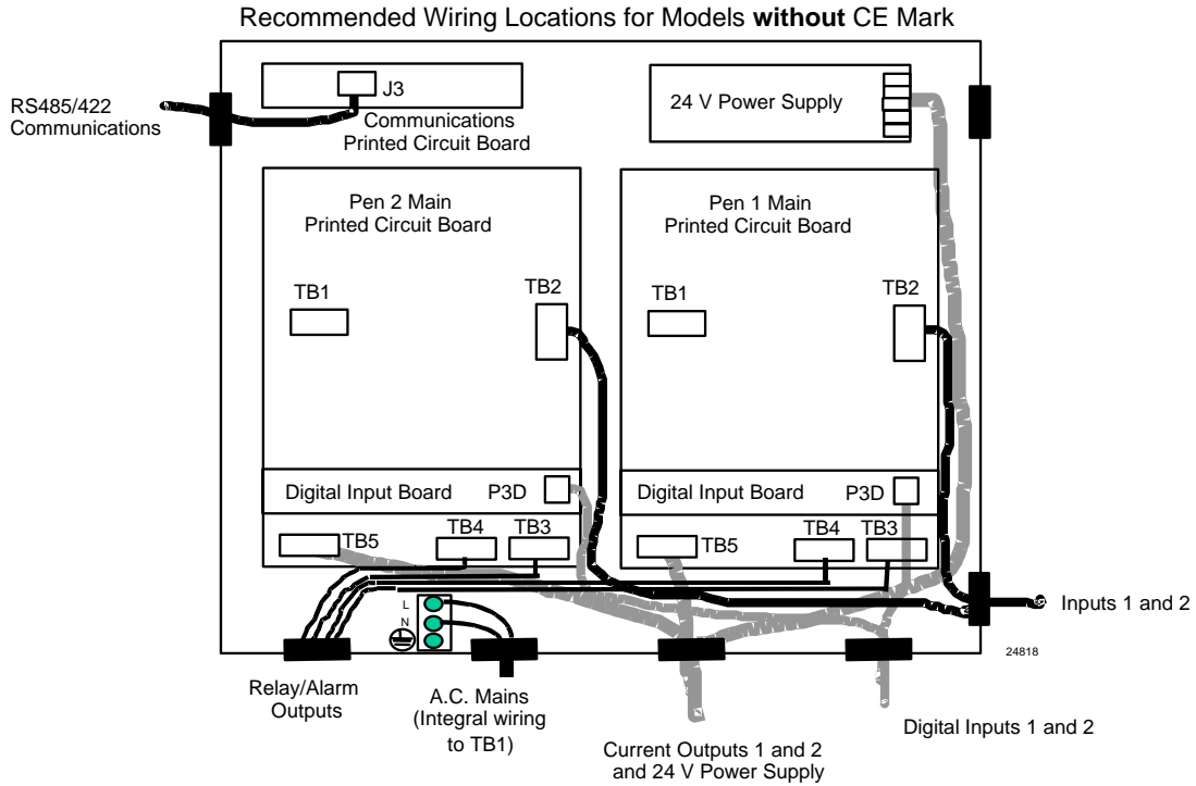
Figure 2-7 Recommended Wiring Routing - Models Without CE Mark
