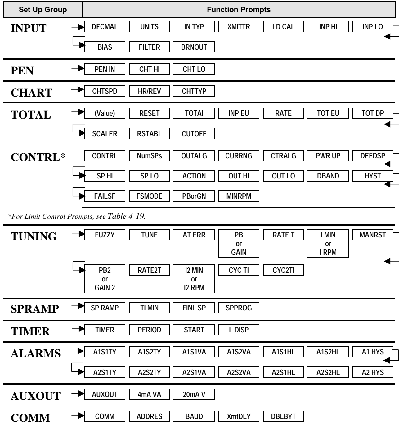
Figure 4-2 Prompt Hierarchy
