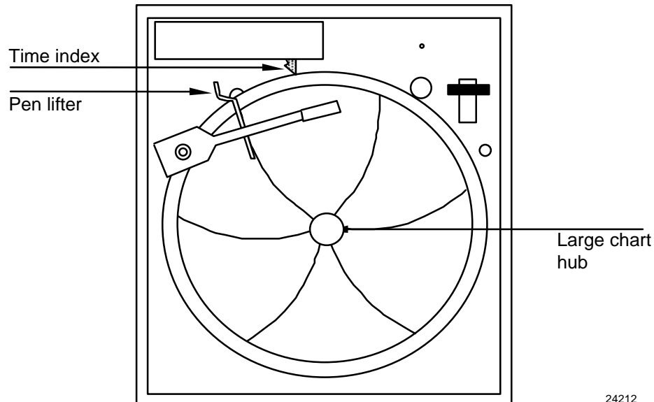
Figure 3-5 Setting Chart Time to Time Index
